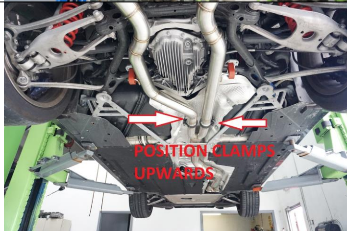
19. SNUG BALL CLAMPS (13MM) WITH BOLT END TOWARDS BOTTOM OF CAR. WILL NEED TO REPOSITION WHEN REAR EXHAUST ATTACHED.
